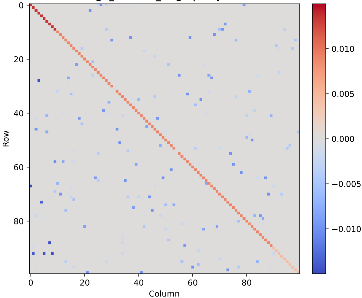
gd_random_large | step 0
